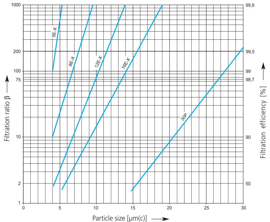
ARGO-HYTOS filter fineness: filtration ratio \beta and filtration efficiency in relation to particle size to ISO 16889
