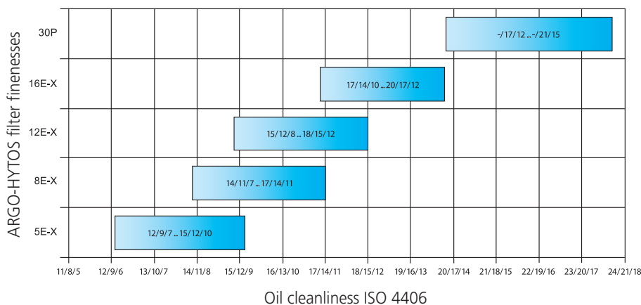
Attainable oil cleanliness levels
