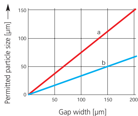
Permitted particle size in relation to gap width with (a) large and (b) small relative movement of the gap surfaces.
