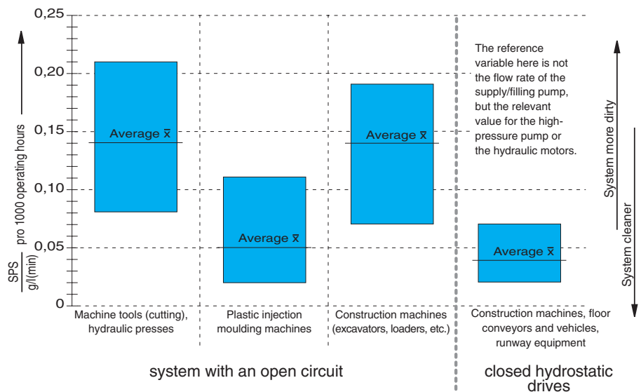
SPS values for typical hydraulic systems
