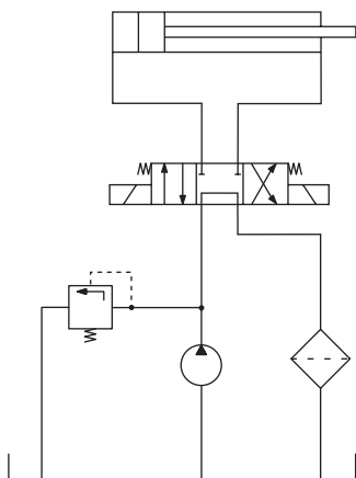
Hydraulic system with return filter
