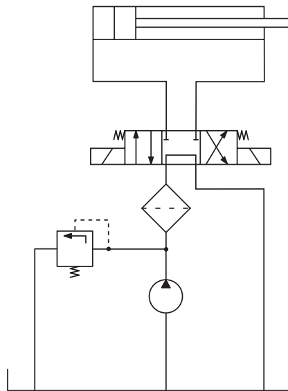
Hydraulic system with high-pressure filter
