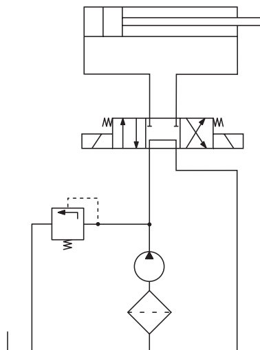
Hydraulic system with suction filter
