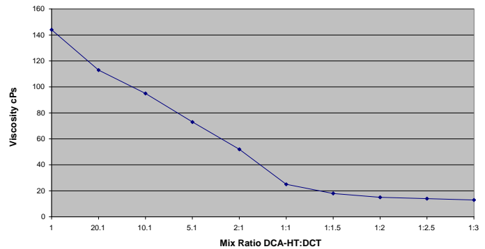
Viscosity Chart DCA-HT:DCT
