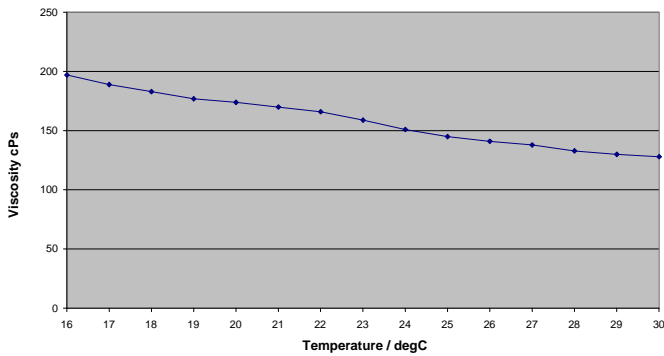
Viscosity Change with Temperature – DCA-HT
