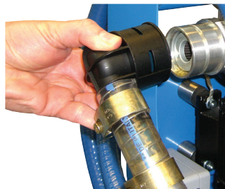
FA 016 with screwed-in suction strainer set FA 016.1775
