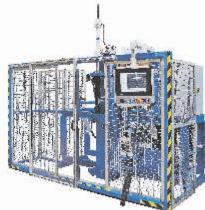
Shock Absorber Test Machine
